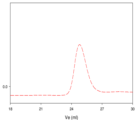
Size Exclusion Chromatography for P8052-LA2OH (DL form) Mn =6900 and PDI =1.15
