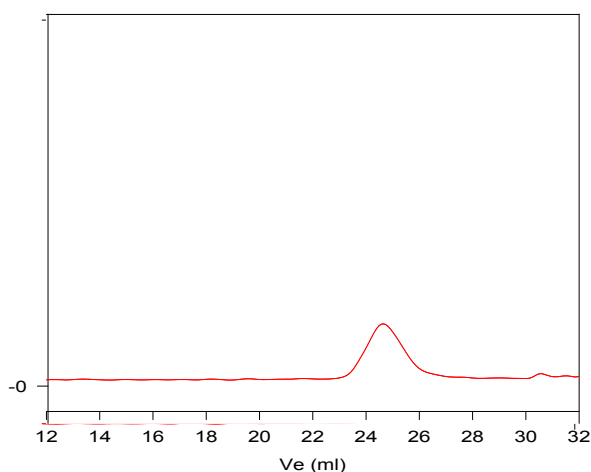
Size exclusion chromatograph of Poly lactide diol (dLform) lot # P8235 Mn: 6500 Mw: 7500 Mw/Mn 1.15 from 1 H NMR Mn: 7000
